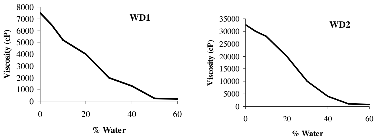
Figure 5. Viscosity change with the addition of water for WD1 and WD2
