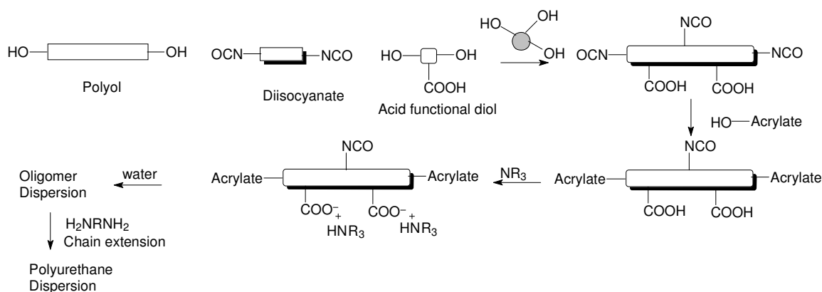
Figure 1. Preparation of UV-PUDs
