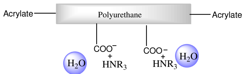
Figure 2. Acid-amine stabilized WR-UAs.
