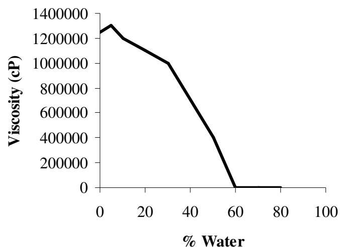
Figure 3. Viscosity change with the addition of water for WR3
