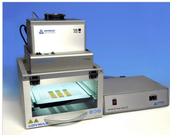
Figure 1. Dymax 2000-EC Curing System
