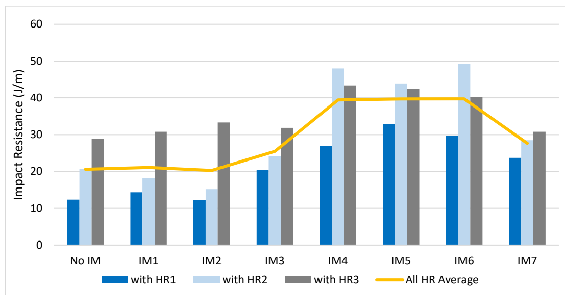
Figure 3. Formulation Impact Resistance
