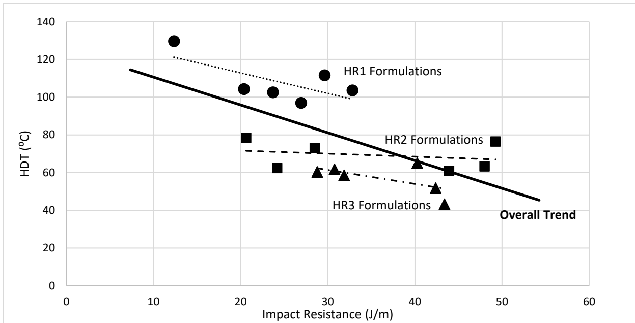
Figure 7. Relationship between HDT and Impact Resistance
