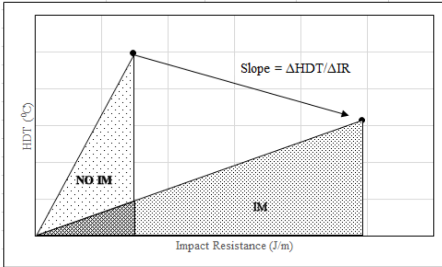
Figure 8. Impact Resistance-HDT Trade-Off Analysis Parameters
