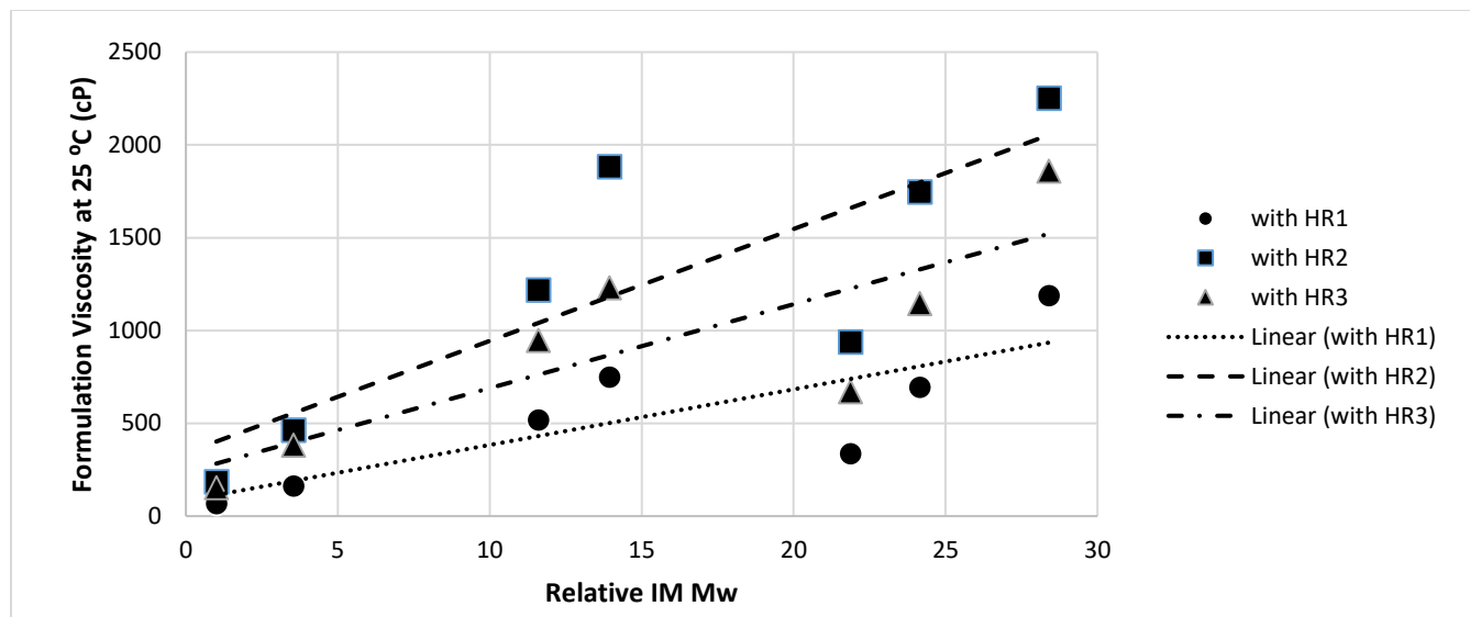
Figure 2. Relationship between IM Molecular Weight and Formulation Viscosity. R^2 Value for all linear trends is 0.66 \pm 0.01 .
